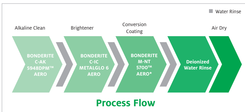
Repaint – Metal pretreatment for spray application
